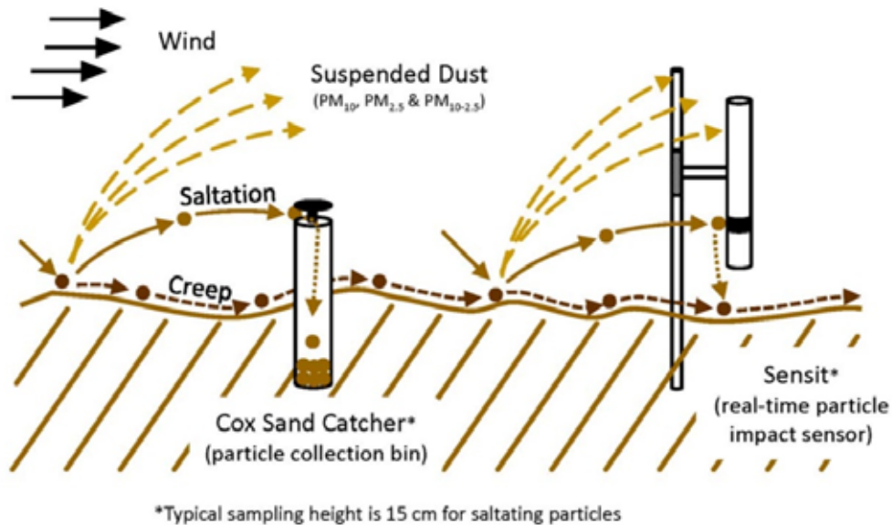
FIGURE 2-6 Illustration of sand flux monitoring site using a Cox Sand Catcher to collect sand-sized particles and Sensit that detects saltating particles. SOURCE: EPA, 2019b.
