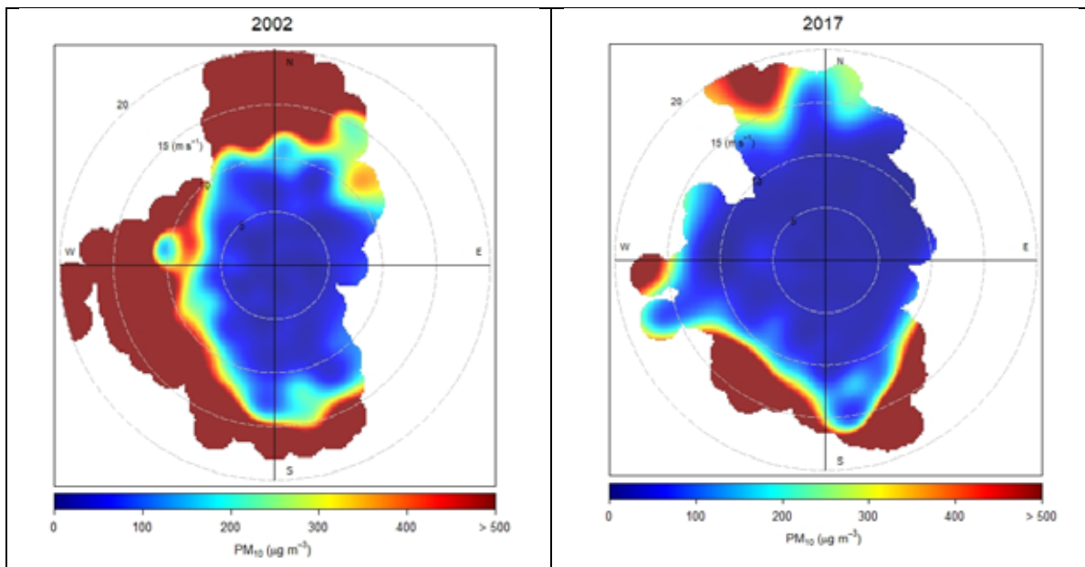
FIGURE 2-9 PM 10 -Wind velocity plots for the Dirty Socks monitoring site in 2002 and 2017 constructed using hourly PM 10 concentrations.
