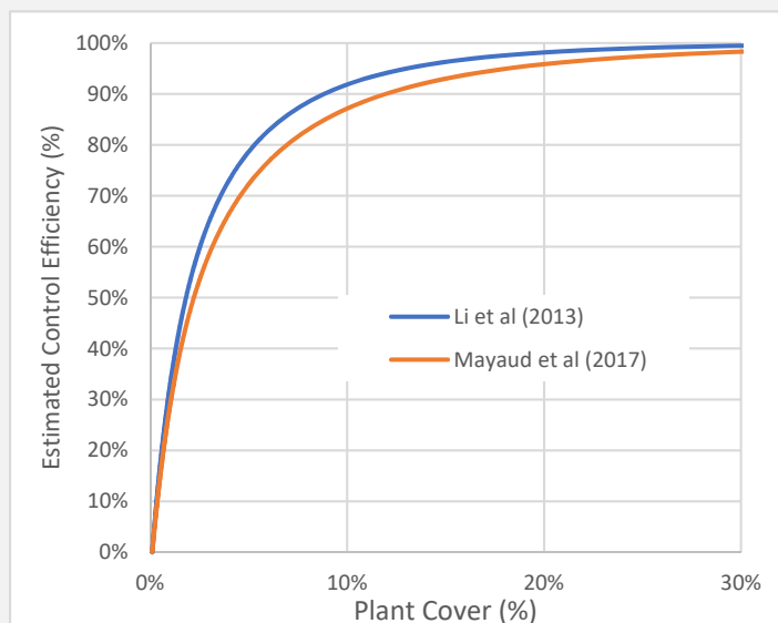
FIGURE A Estimated control efficiency (CE) using two sets of parameters in the Okin (2008) model using 5-minute winds from North Beach, assuming gamma distribution of plant spacing and plant height = plant diameter = 50 cm.
