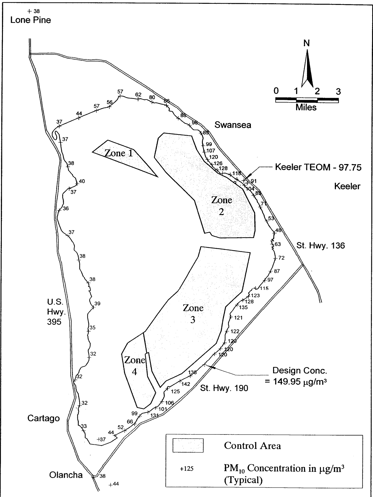
Figure 8: Air quality model: third highest 24-hour PM_{10} concentrations for 1994-95 with controls in place.
