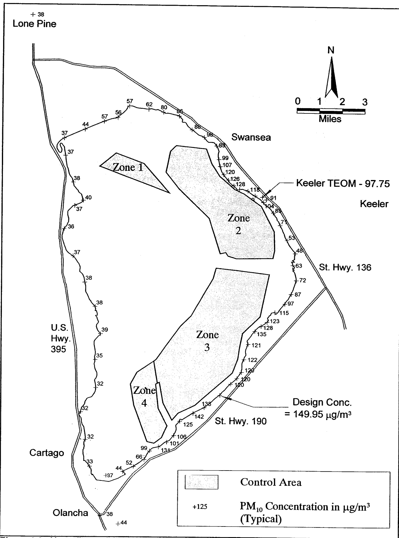
Figure 6.3: Air quality model: third highest 24-hour PM_{10} concentrations for 1994-95 with controls in place.
