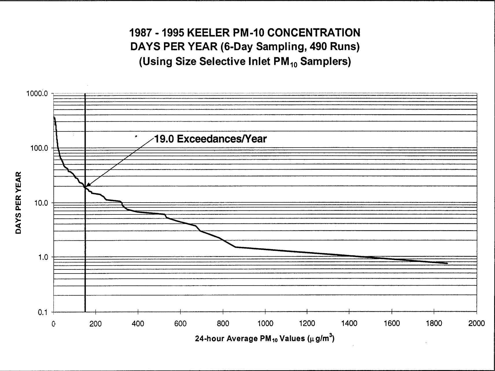
Figure 3.4: Keeler PM 10 frequency distribution shows that PM 10 levels exceed the 150µg/m 3 24-hour NAAQS about 19 days per year.
