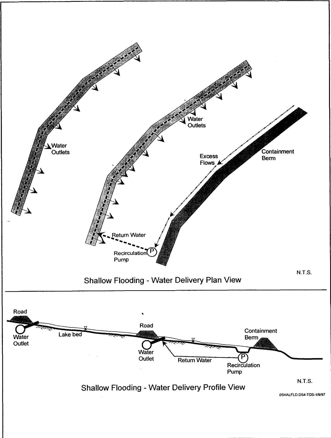
Figure 5.2: Shallow flooding - water delivery schematic.
