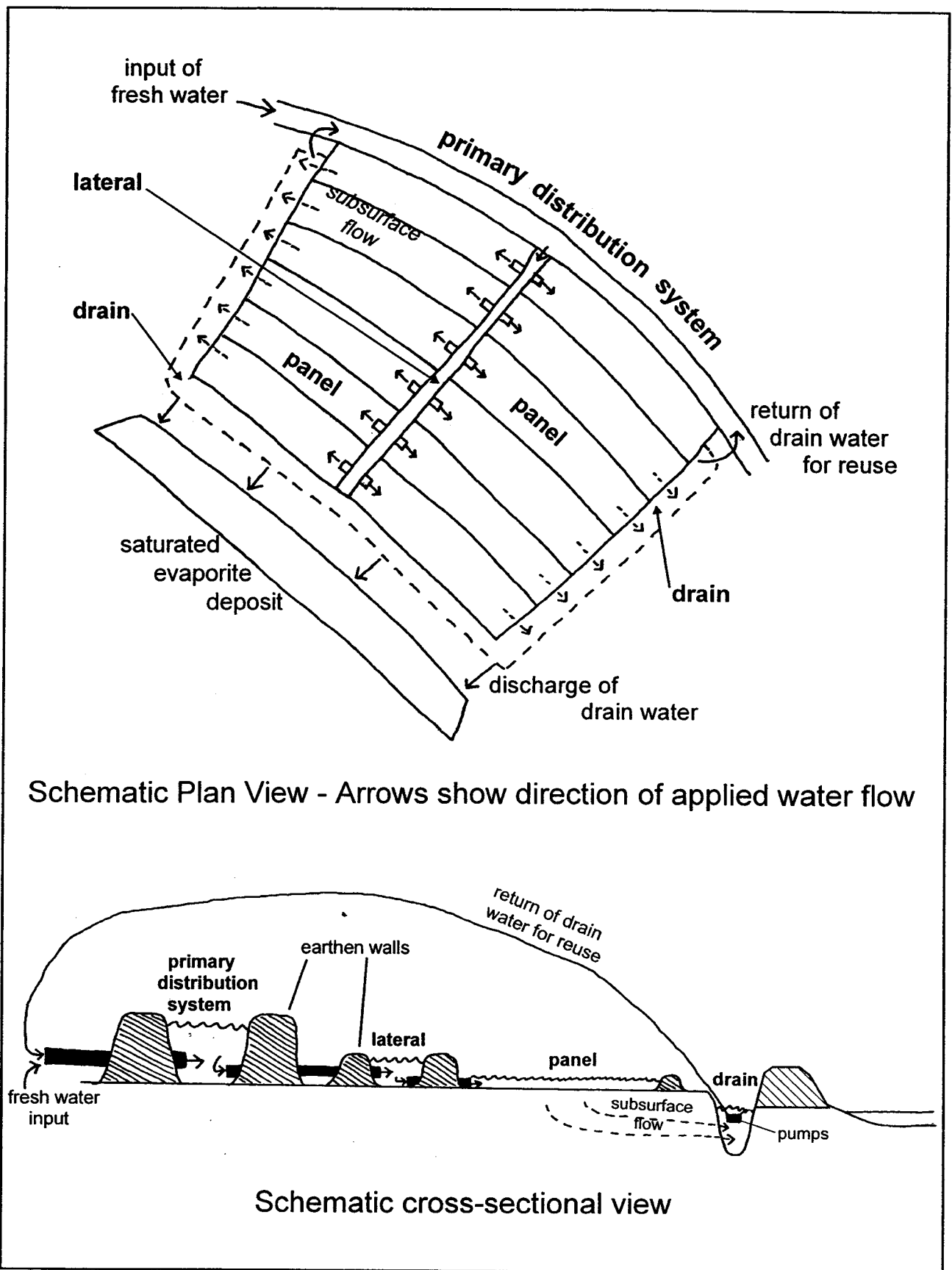
Figure 5.6: Managed vegetation - water delivery schematic.
