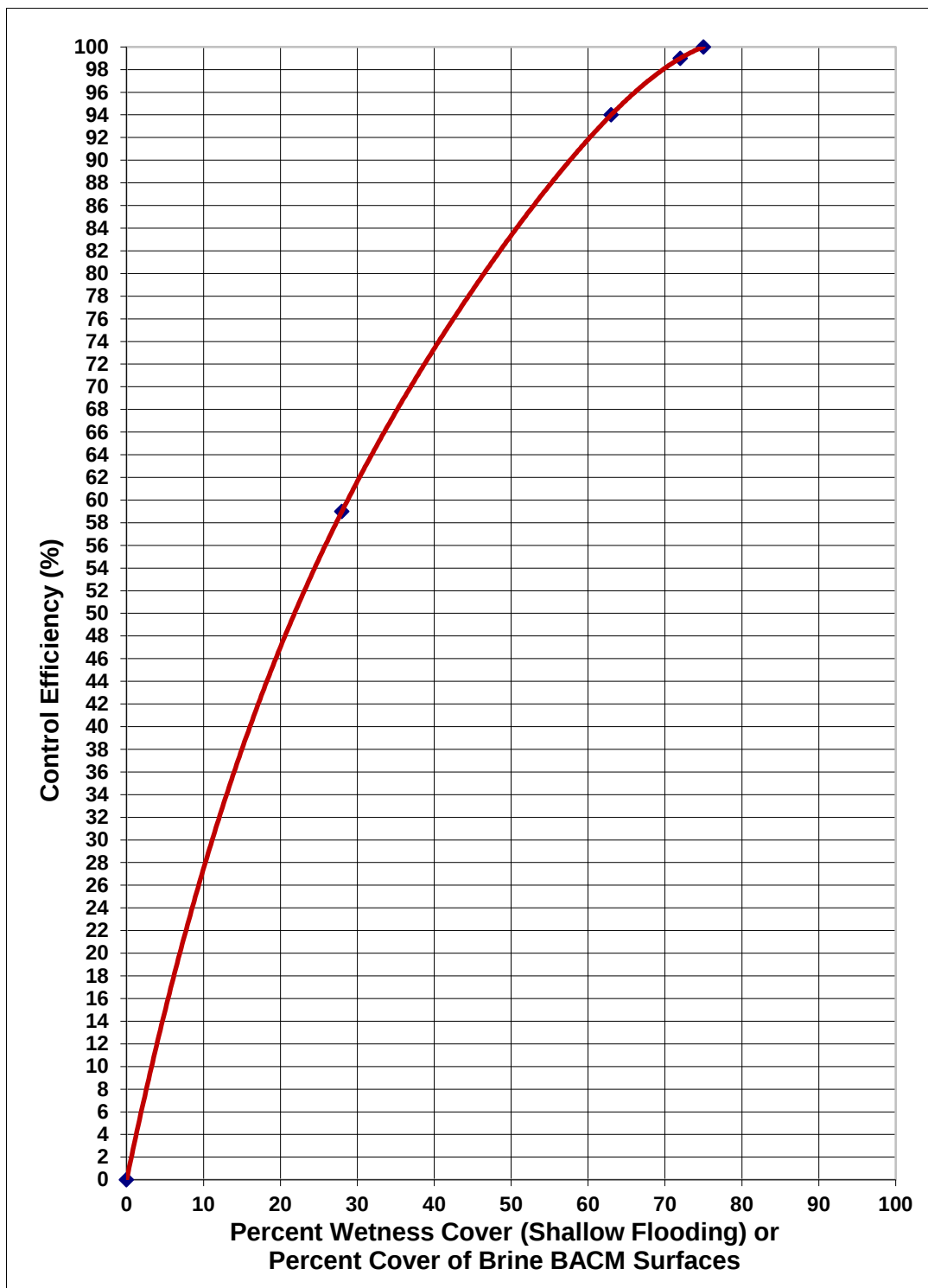
Figure A1. Shallow Flooding control efficiency wetness cover curve used to determine the percentage of surface cover required for the three qualifying stable surfaces that are part of Brine BACM.
