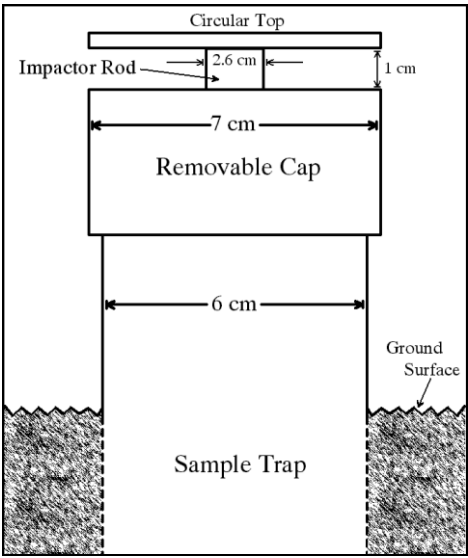
Figure C.2.2 - Diagram of the Cox Sand Catcher (CSC) used to measure sand flux at Owens Lake.
